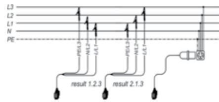
Circuit for voltage measurement, frequency and phase sequence
