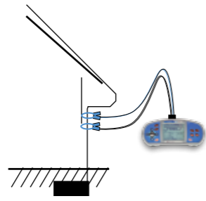
Two clamps method
